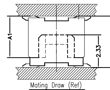
**Mating Dimension
