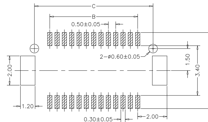
PCB LAYOUT
