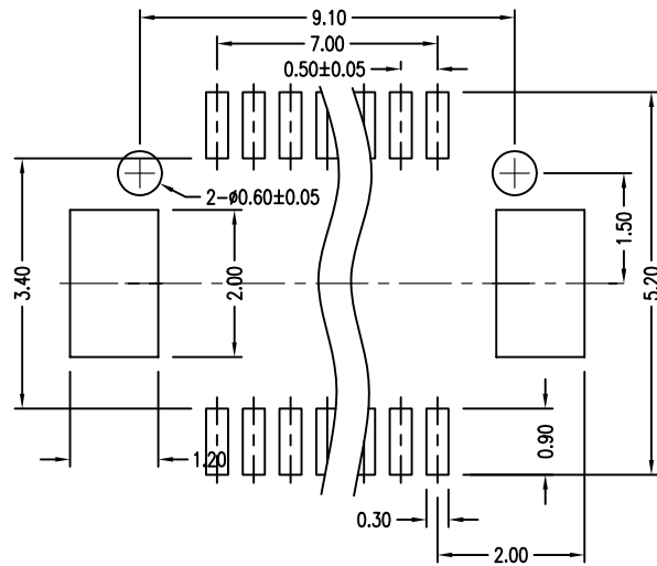
PCB LAYOUT
