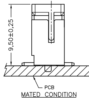
PCB MATED CONDITION
