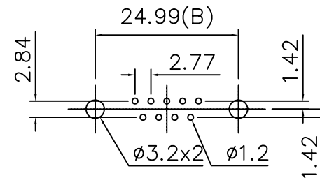
Recomended PCB Layout
