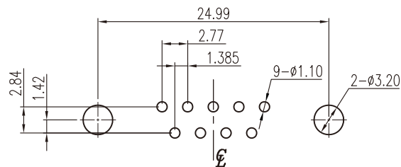
RECOMMENDED P.C.B LAYOUT INSPECTION DIMENSION:(A)~(F)
