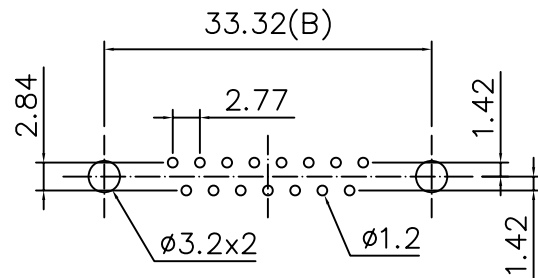
Recomended PCB Layout
