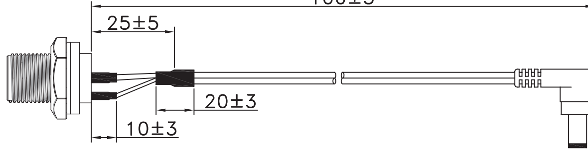
DC JACK PANEL
