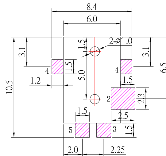
P.C.B LAYOUT MOUNTING PATTERN (TOP VIEW)
