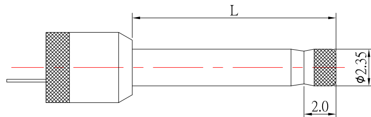
RECOMMENDED PLUG
