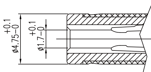
MATED PLUG
