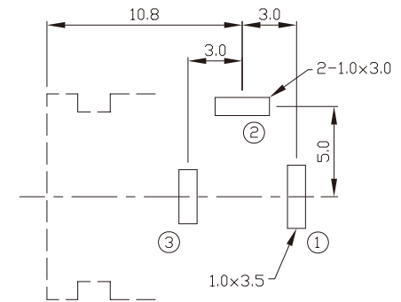
PCB LAYOUT(±0.1) (BOTTOM VIEW)
