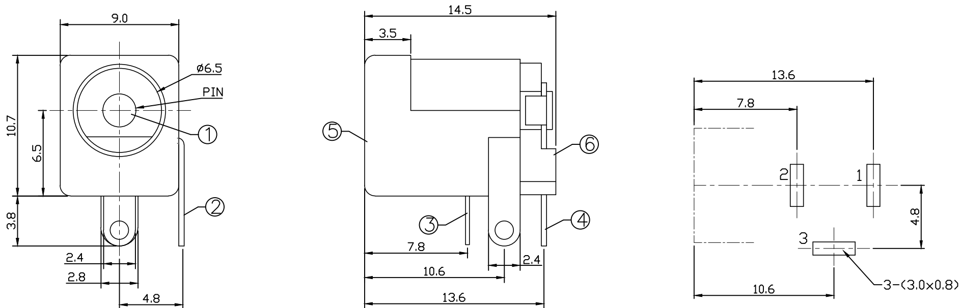
T:1.6 Dimensions of PC board holes Tolerance : ±0.05(Printed-top view)
