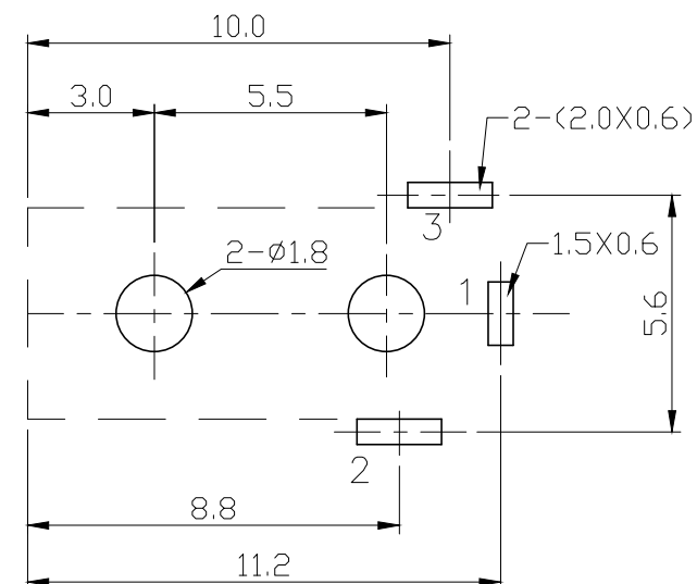
T:1.6 Dimensions of PC board holes
