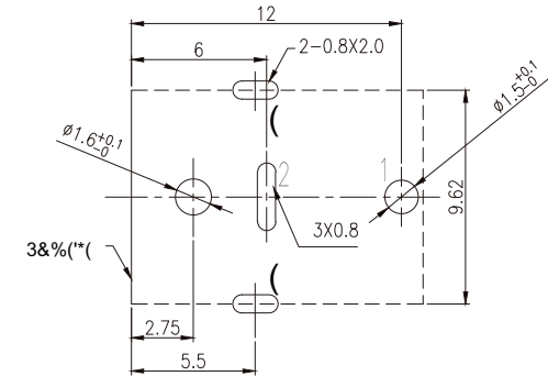
MATE PLUG Ø5.5
