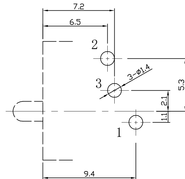
T:1.6 Dimensions of PC board holes Tolerance : \pm 0.05 (Printed-top view)
