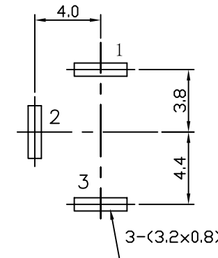
T:1.6 Dimensions of PC board holes Tolerance : \pm 0.05 (Printed-top view)
