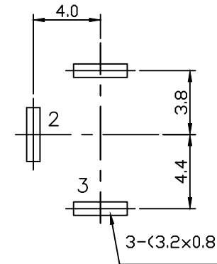
T:1.6 Dimensions of PC board holes Tolerance : \pm 0.05 (Printed-top view)
