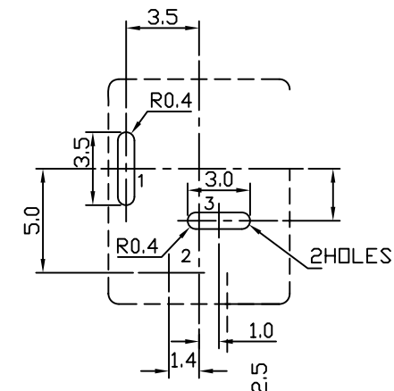
T:1.6 Dimensions of PC board holes
