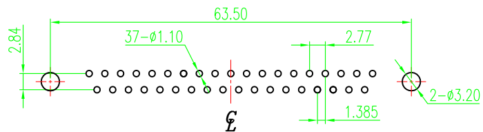
RECOMMENDED P.C.B. LAYOUT INSPECTION DIMENSION:(A)~(F)
