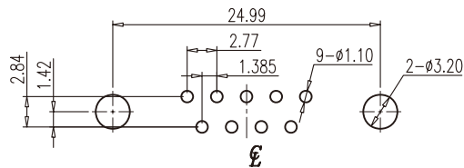
RECOMMENDED P.C.B LAYOUT INSPECTION DIMENSION:(A)~(G)
