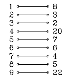
WIRING DIAGRAM D-SUB-09P D-SUB-25P
