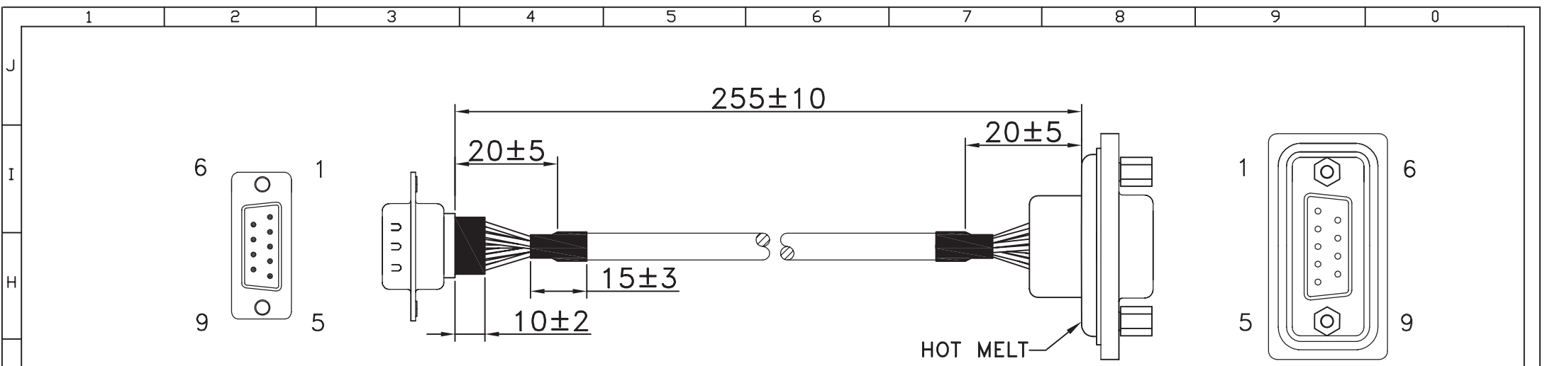
FRONT VIEW
