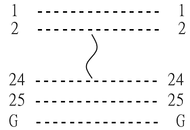
DB 25 M/M GENDER CHANGER PIN OUT: 25Male
