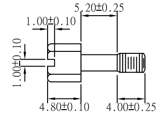
UNC #4-40 Hexscrew
