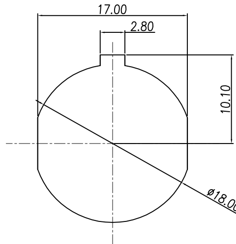
Panel Cut-Out
