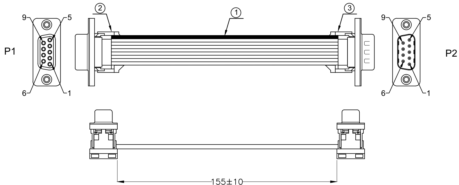
WIRE DIAGRAM
