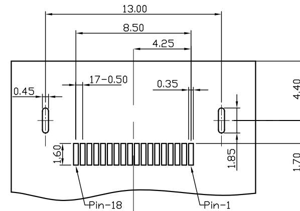
P.C BOARD LAYOUT (TOLERANCE: \pm 0.05\text{mm} )
