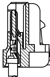
Mated Drawing(REF.)
