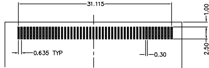
Recommend PCB Layout
