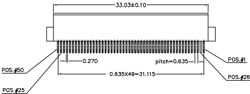
A Picture DETAIL "A" S=4:1
