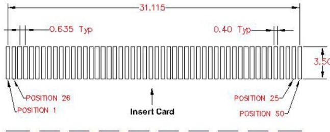
PCB LAYOUT
