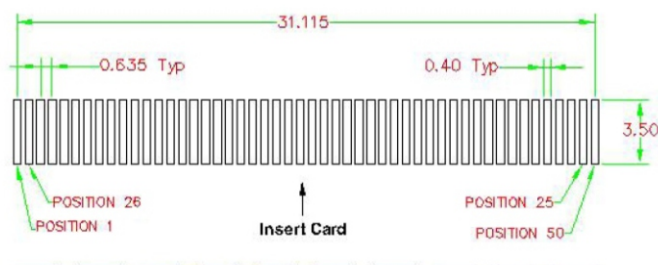
PCB LAYOUT
