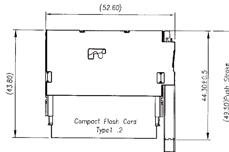
Header With Ejector
