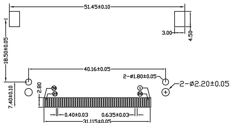
RECOMMENDED LOWER BOARD P.C.B LAYOUT
