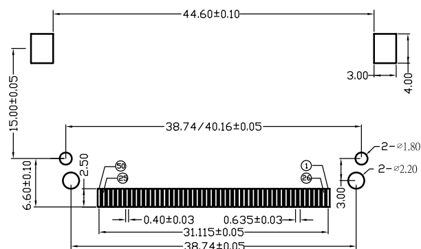
RECOMMENDED UPPER BOARD P.C.B LAYOUT
