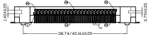
LOWER BOARD
