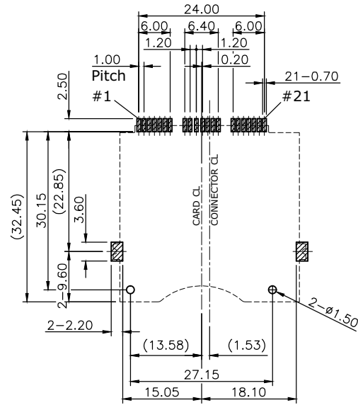
RECOMMENDED LAYOUT(TOP VIEW)
