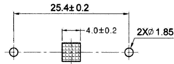
PCB Mounting layout
