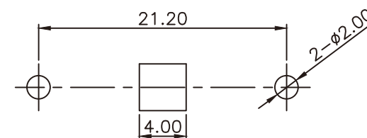
PCB LAYOUT
