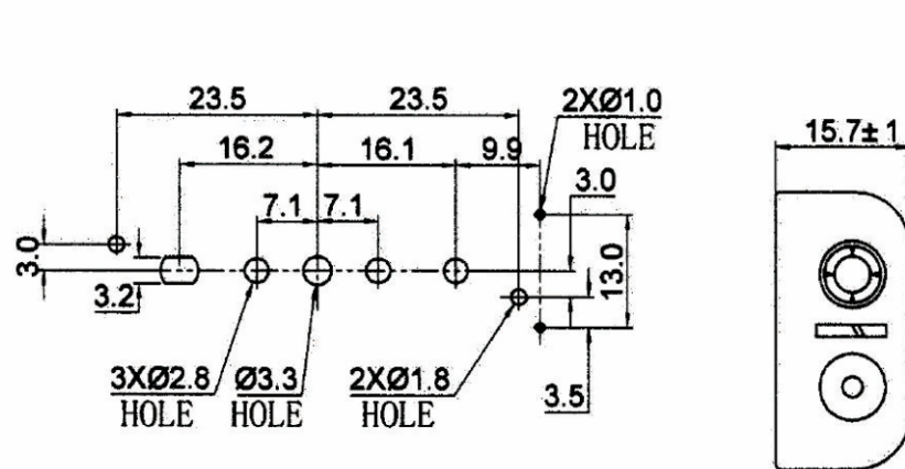
PCB/MOUNTING LAYOUT
