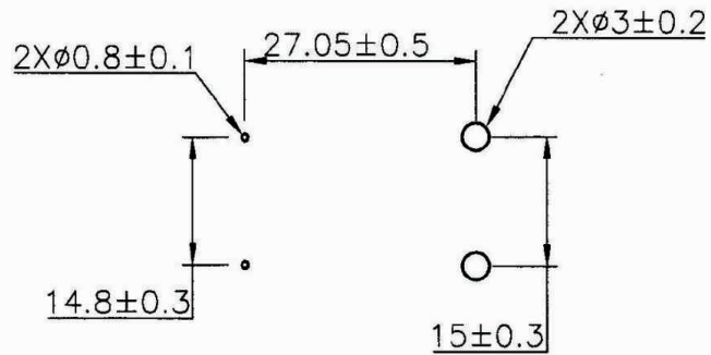
PCB/MOUNTING LAYOUT
