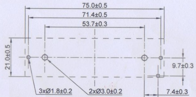
PCB/MOUNTING LAYOUT
