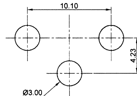
PCB Mounting Layout
