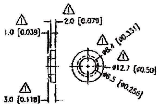
INSULATED WASHER
