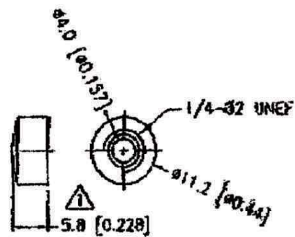
INSULATED HEAD
