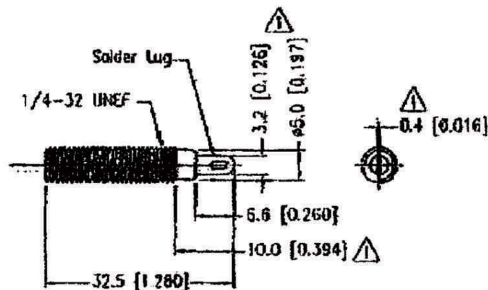
THREADED BODY
