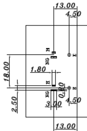
PCB LAYOUT
