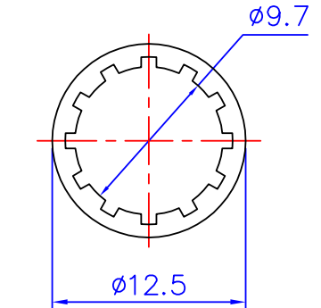
⑥ LOCK WASHER
