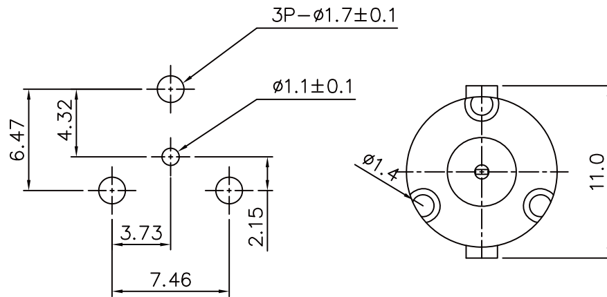
PCB HOLE CONFIGURATION RECOMMENDED PANEL CUTOUTS
