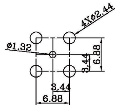
RECOMMENDED PCB LAYOUT (BOTTOM VIEW)
