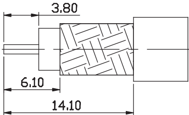
RECOMMEND CABLE STRIPPING
