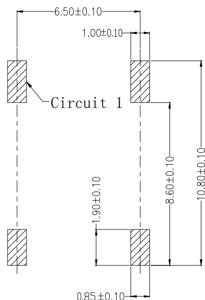
SUGGESTED PCB LAYOUT (COMPONENT SIDE)
