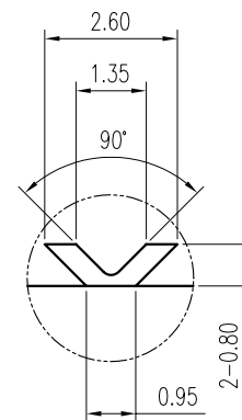
Detail A Scale 6:1
