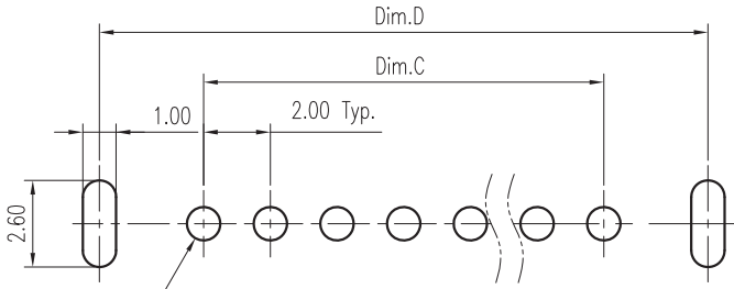
Recommended P.C.B. Layout Layout Tolerance = ± 0.05 mm
