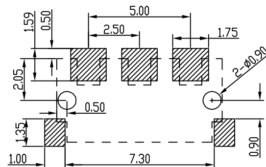
RECOMMENDED PCB. BOARD LAYOUT
